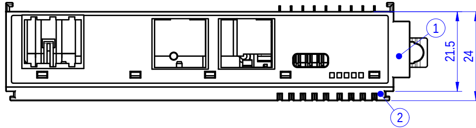
Assembly diagram
