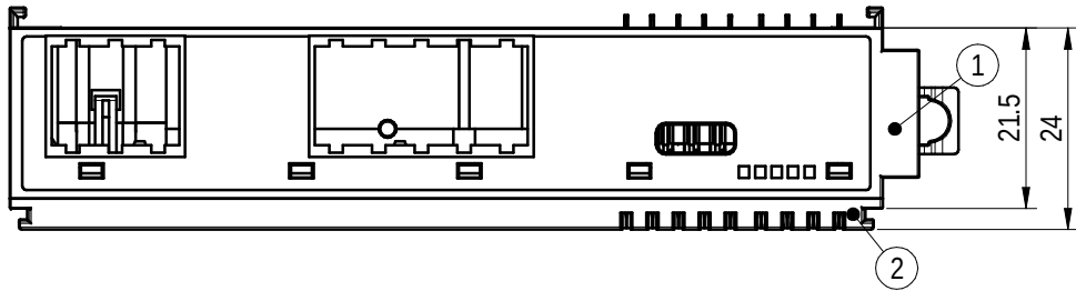
Assembly diagram
