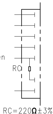
Wiring diagram
