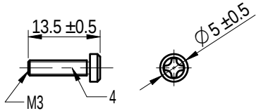
SCREW-1
