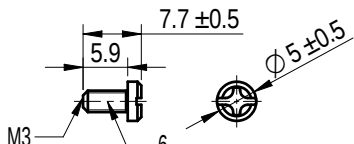
SCREW-2
