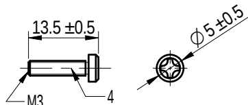
SCREW-1
