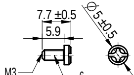
SCREW-2
